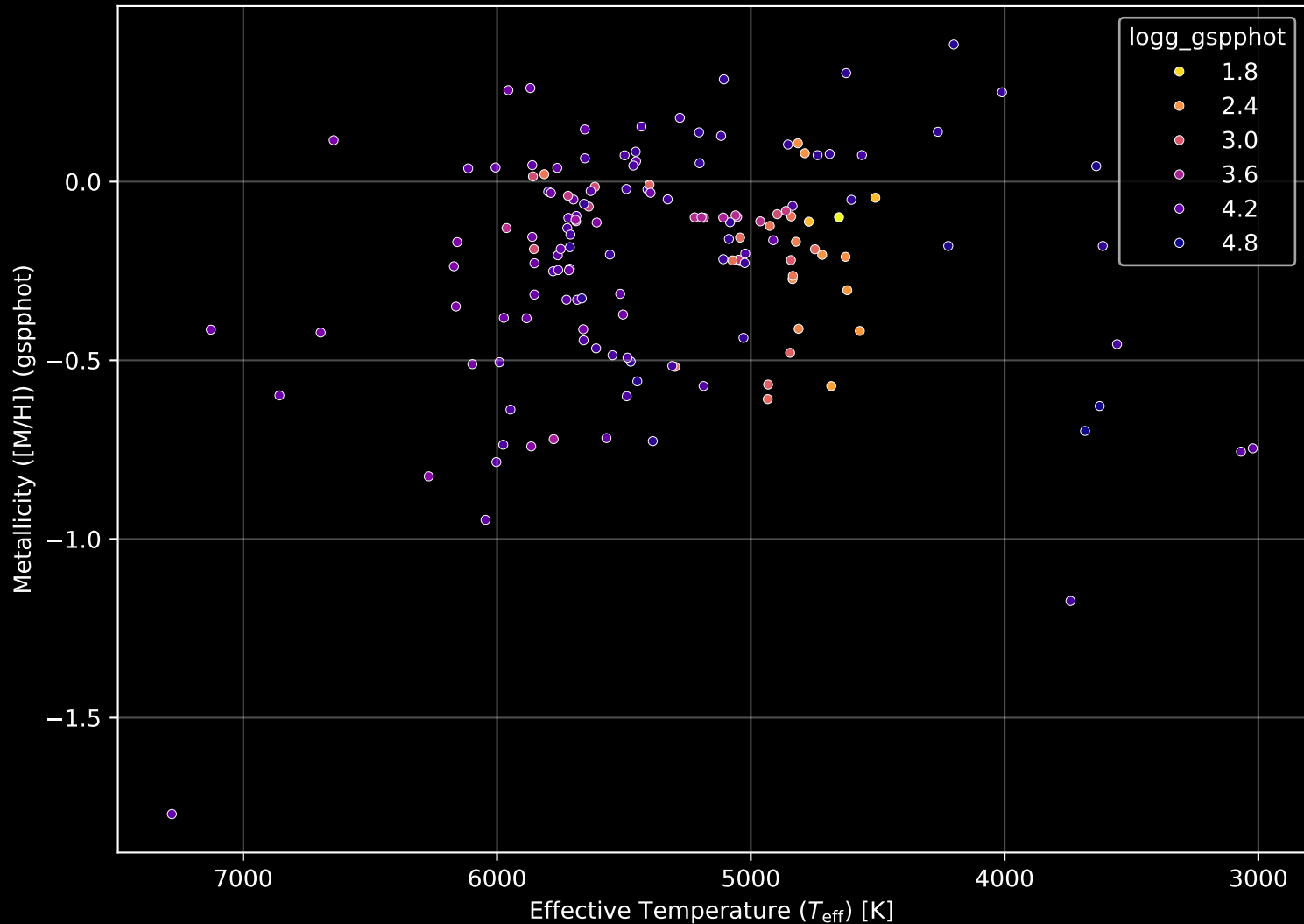
APOGEE DR17 Field: [047+50_MGA] Stellar Population Parameters (n= 150)
