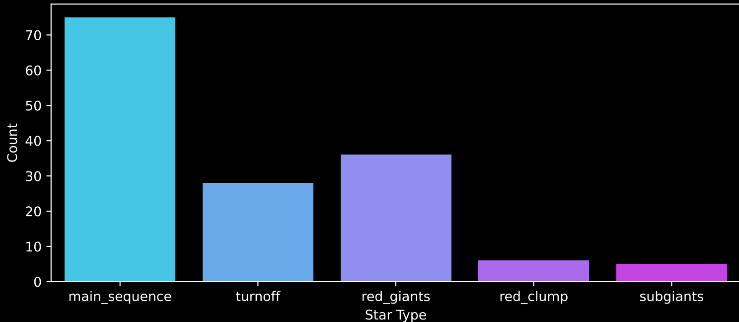
APOGEE DR17 Field: [047+50_MGA] Count plot of Star Type
