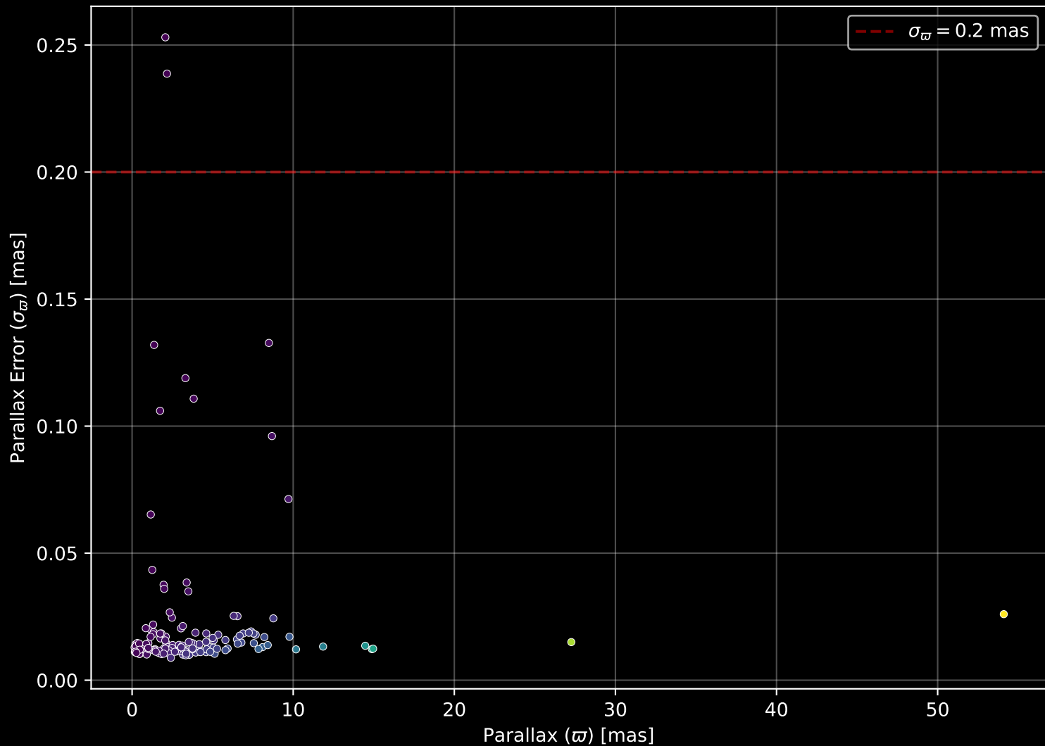
APOGEE DR17 Field: [047+50_MGA] Parallax Quality (n= 150)
