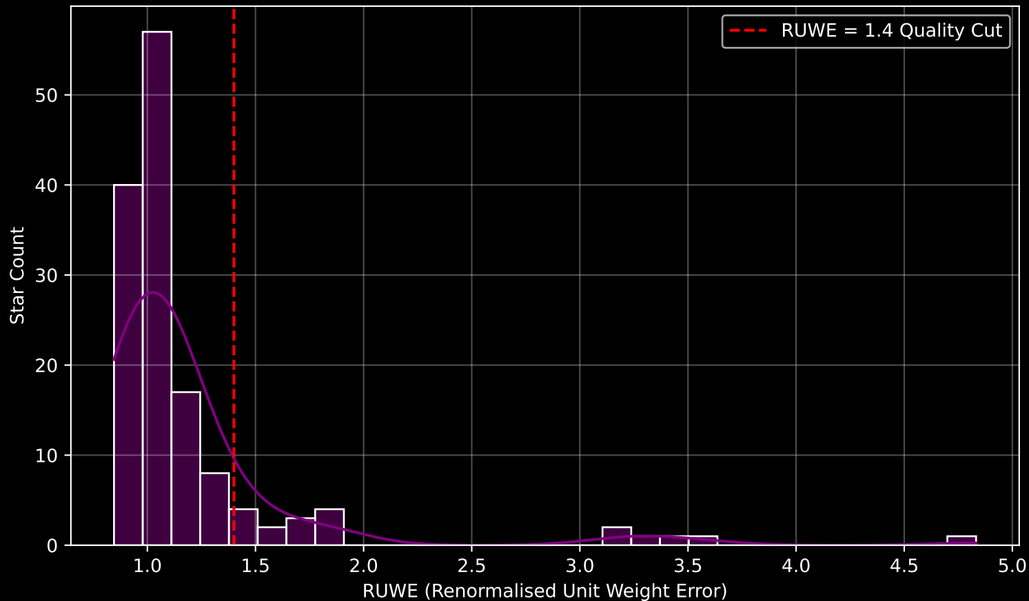
GAPOGEE DR17 Field [047+50_MGA] RUWE Distribution (n= 141)
