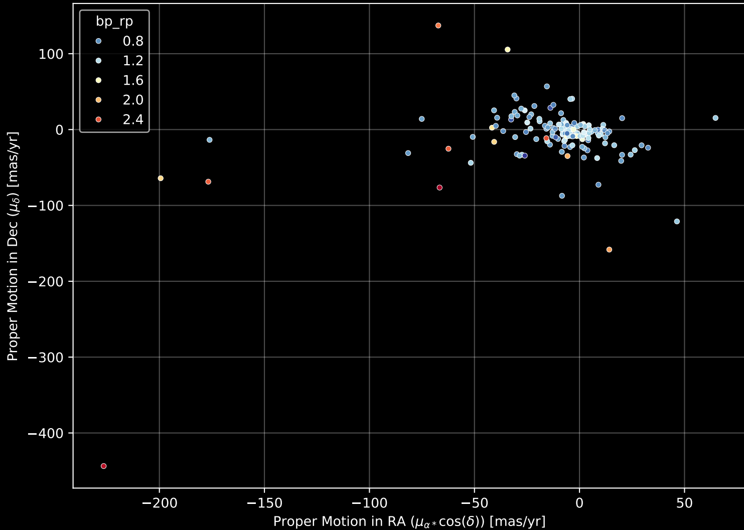
APOGEE DR17 Field: [047+50_MGA] Proper Motion Diagram (n= 150)
