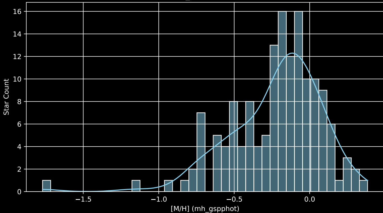
APOGEE DR17 Field: [047+50_MGA [M/H] (mh_gspphot) (n= 150)
